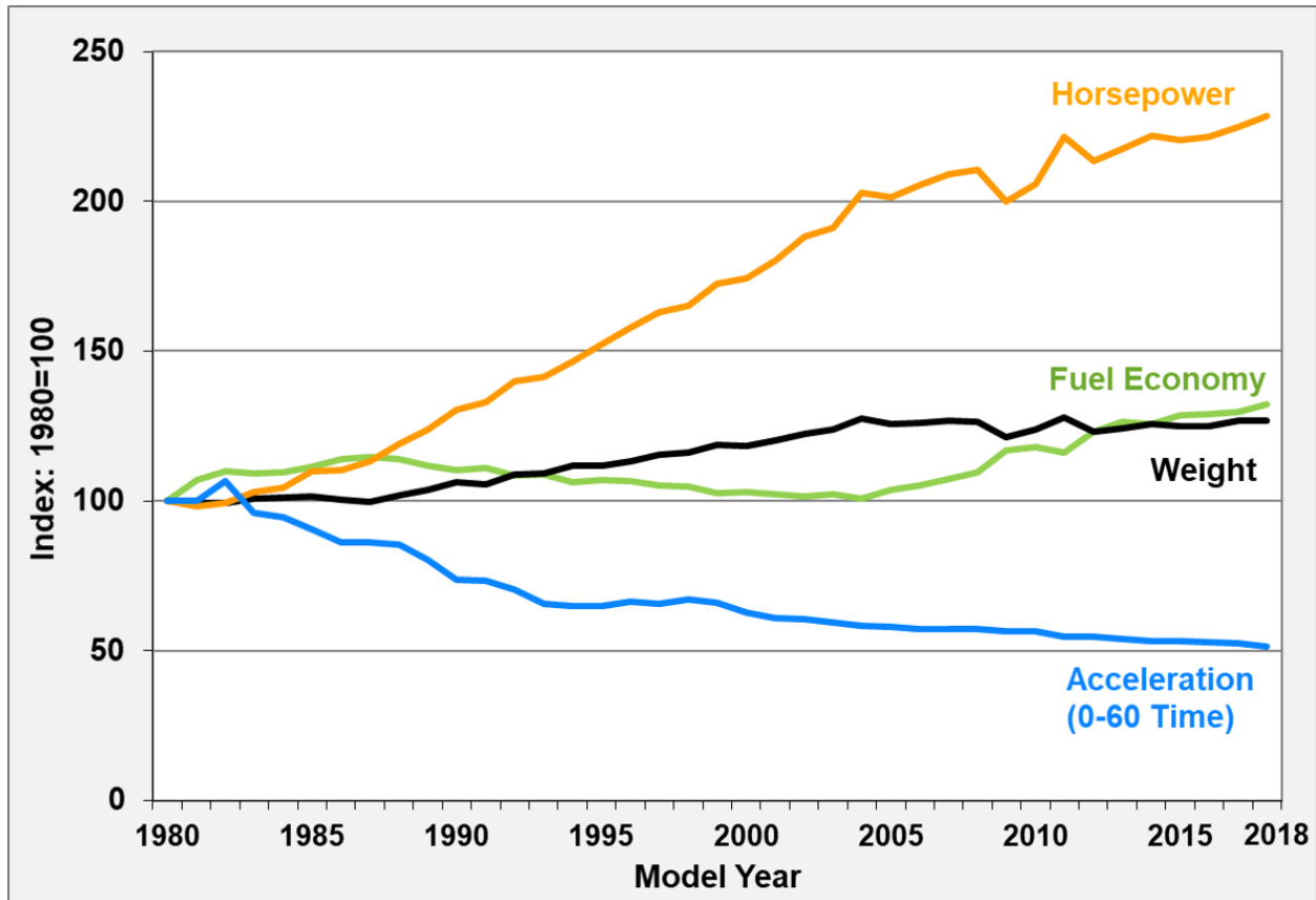
Figure 4.6. Horsepower, Fuel Economy, Weight, and 0-60 Time for New Light Vehicles, Model Years 1980-2018 (Updated April 2019)
