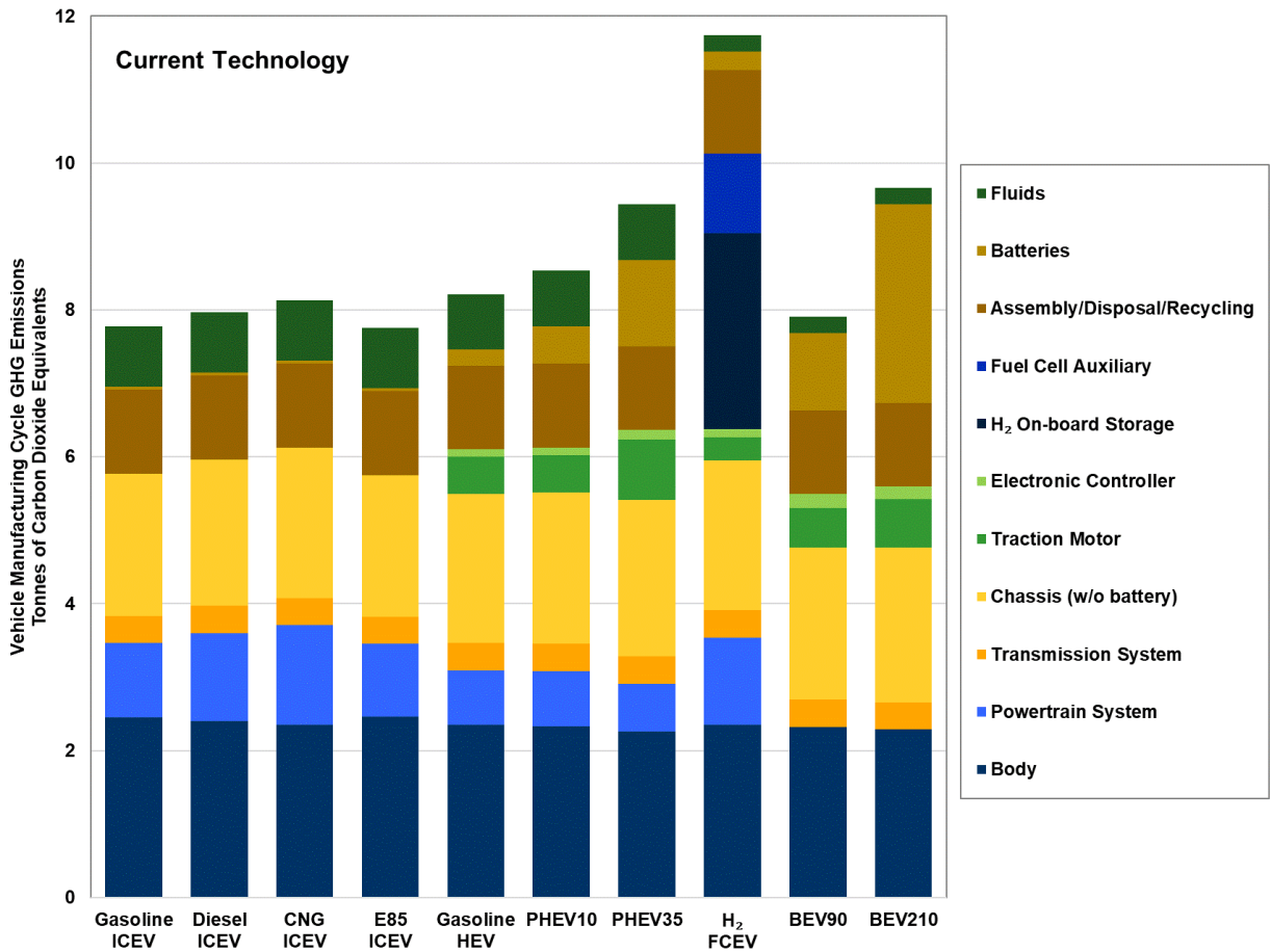
Figure 11.5. Vehicle Manufacturing Cycle Greenhouse Gas Emissions by Vehicle Component (Updated April 2019)
