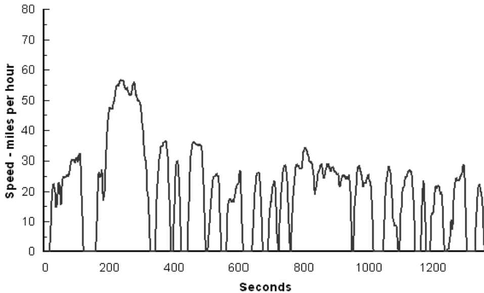
Figure 4.11. Cold Temperature (Cold FTP) Driving Cycle a
